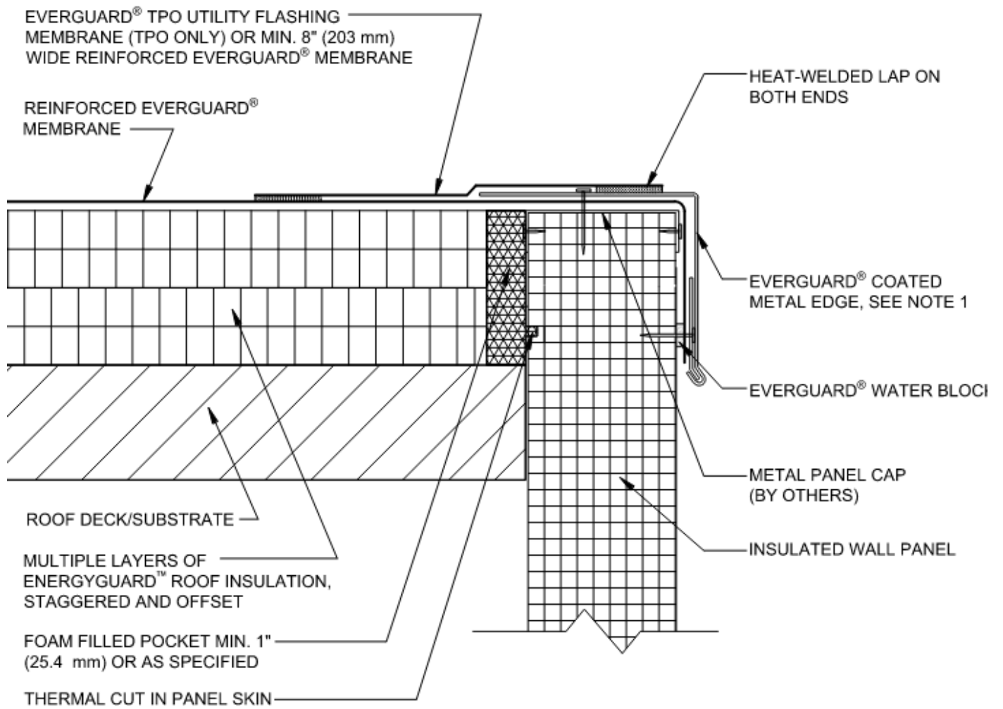
Figure 7: Coated metal roof edge at insulated wall panel, note the installation of closed cell spray foam at the wall to deck intersection. Reference GAF Cold Storage Detail 201C.
